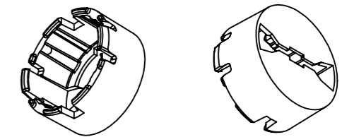
PART VIEW SCALE 1:1
