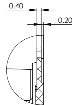
DETAIL D SCALE 5 : 1
