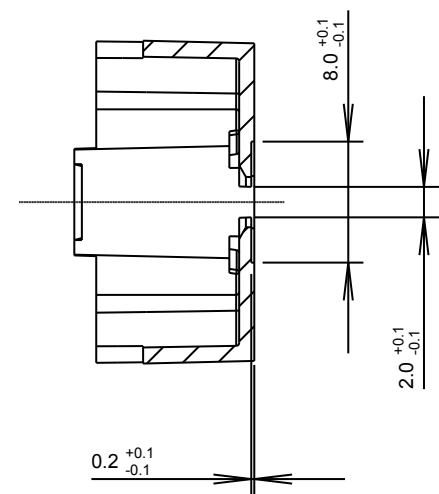
SECTION Y-Y
